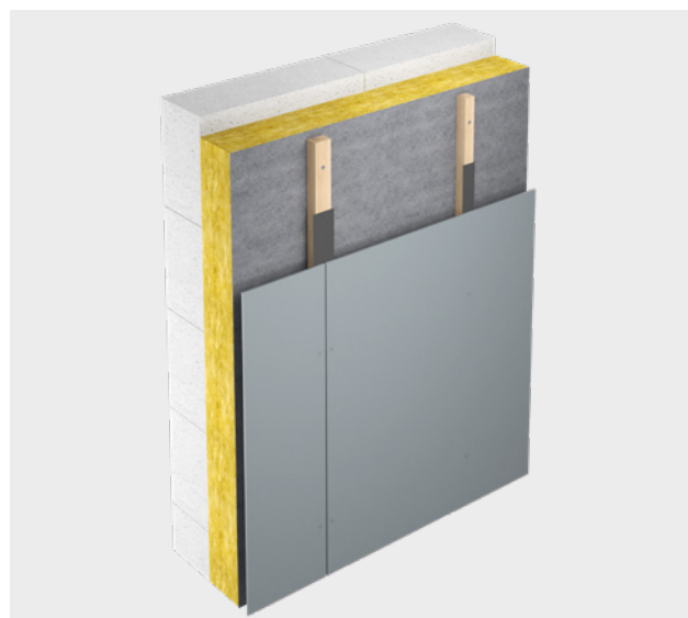
Support battens fixed to the substrate with frame anchors
