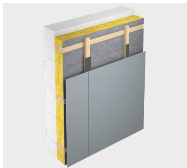
Construction with horizontal counter battens
